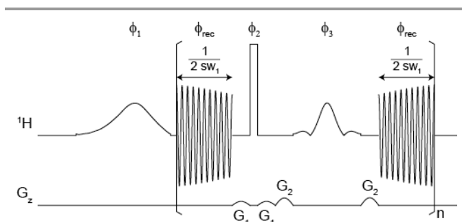
Figure 1: Real time pure shift sequence using a 90^\circ selective excitation pulse (eBURP) with phase \phi_1 , and a J-refocusing element comprising a broadband 180^\circ pulse with phase \phi_2 and a band-selective (rSNOB) 180^\circ refocusing pulse with phase \phi_3 . Data points are collected using a looped, windowed acquisition with phase \phi_{rec} . The J-refocusing and acquisition loop is repeated n times until the required number of data points have been collected. Phase cycle: \phi_1 = x, -x, -x, x, y, -y, -y, y ; \phi_2 = x, -x ; \phi_3 = -x, x ; \phi_{rec} = \phi_1 . The duration 1/sw_1 of the acquisition chunks depends on the balance required between resolution and spectral purity; a good compromise is an sw_1 roughly twice the maximum multiplet width in the normal spectrum.
